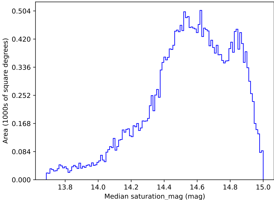
ddf_loaded_half_fl2_v3.4_10yrs All sky r band: Median saturation_mag
