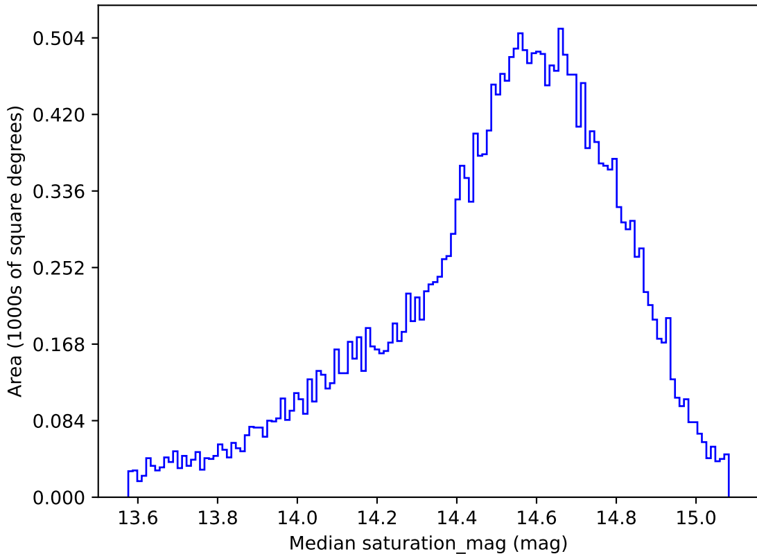
ddf_loaded_half_fl2_v3.4_10yrs All sky g band: Median saturation_mag
