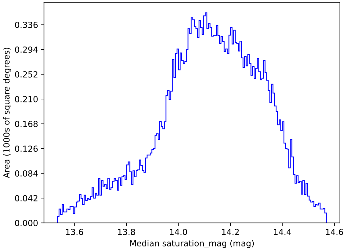
ddf_loaded_half_fl2_v3.4_10yrs All sky all bands: Median saturation_mag
