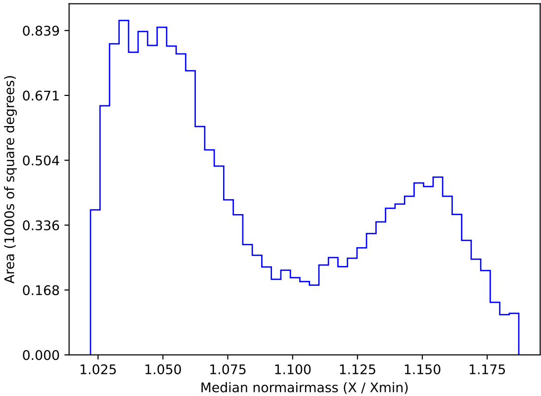
ddf_loaded_half_fl2_v3.4_10yrs WFD z band: Median normairmass
