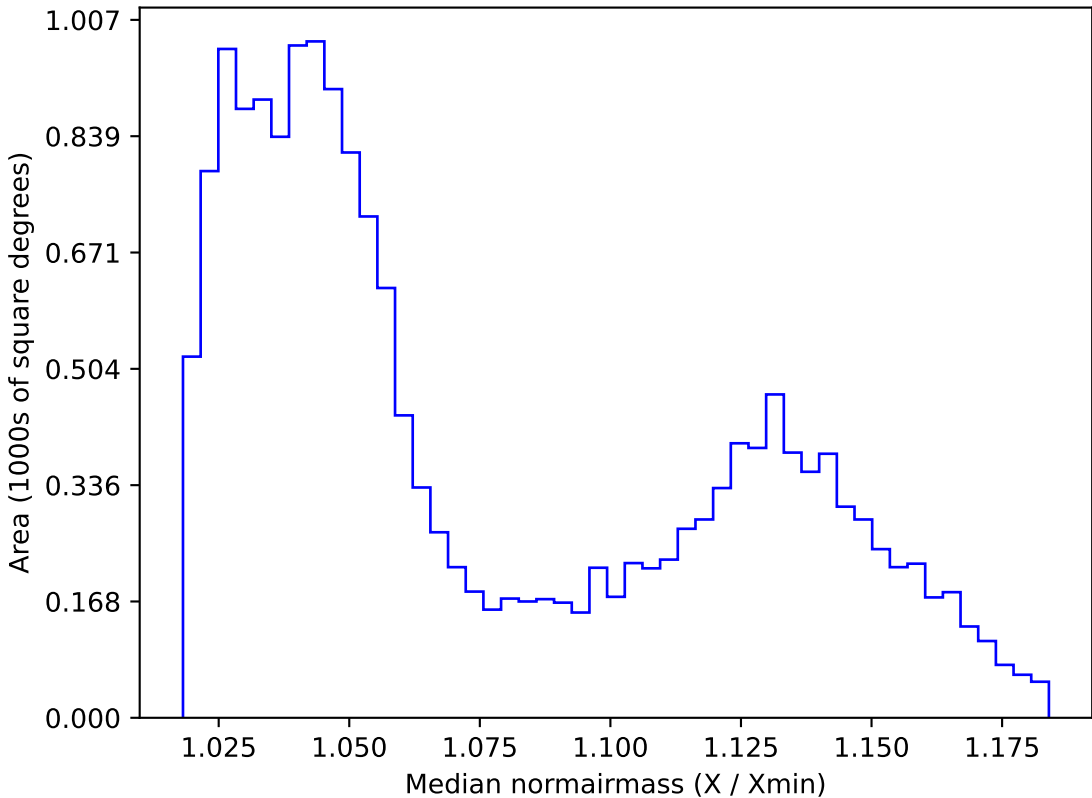
ddf_loaded_half_fl2_v3.4_10yrs WFD r band: Median normairmass
