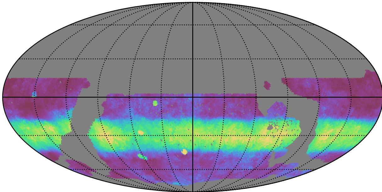
ddf_loaded_half_fl2_v3.4_10yrs WFD i band: Median normairmass
