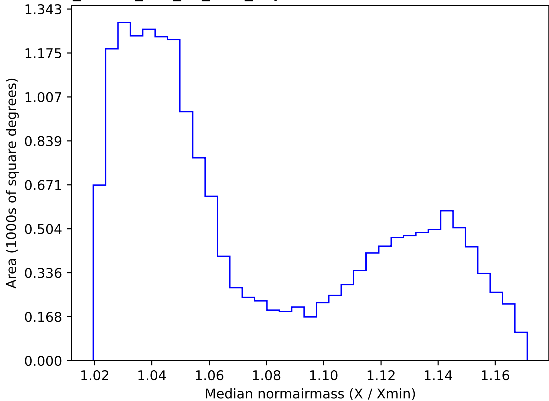
ddf_loaded_half_fl2_v3.4_10yrs WFD i band: Median normairmass
