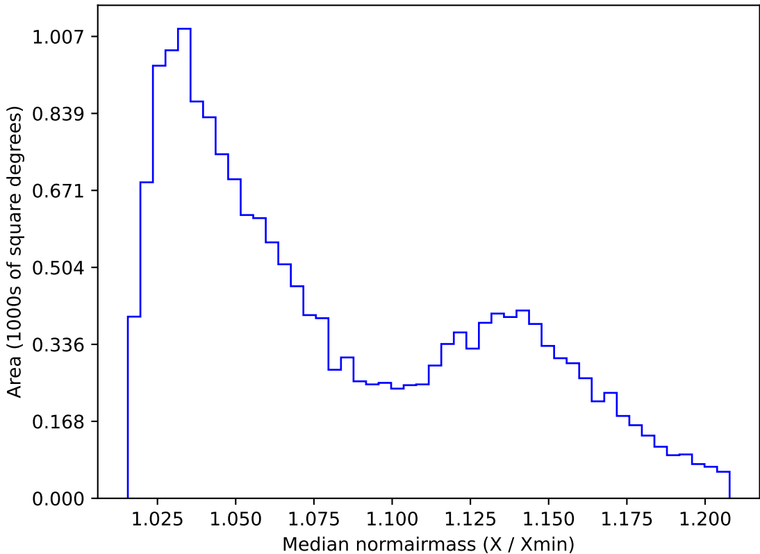
ddf_loaded_half_fl2_v3.4_10yrs WFD g band: Median normairmass
