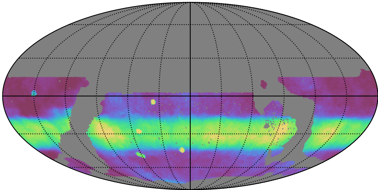
ddf_loaded_half_fl2_v3.4_10yrs WFD all bands: Median normairmass
