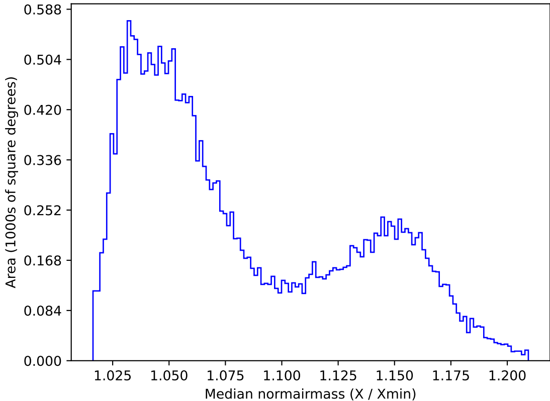
ddf_loaded_half_fl2_v3.4_10yrs All sky z band: Median normairmass
