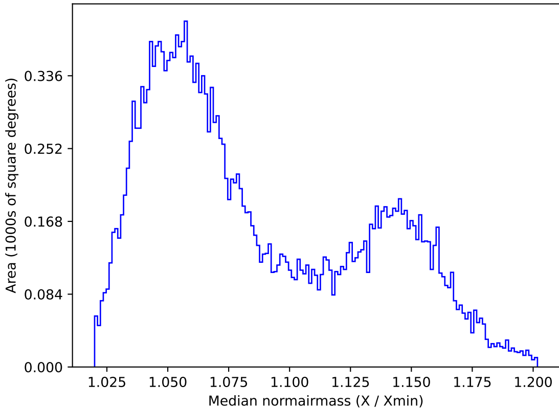
ddf_loaded_half_fl2_v3.4_10yrs All sky y band: Median normairmass
