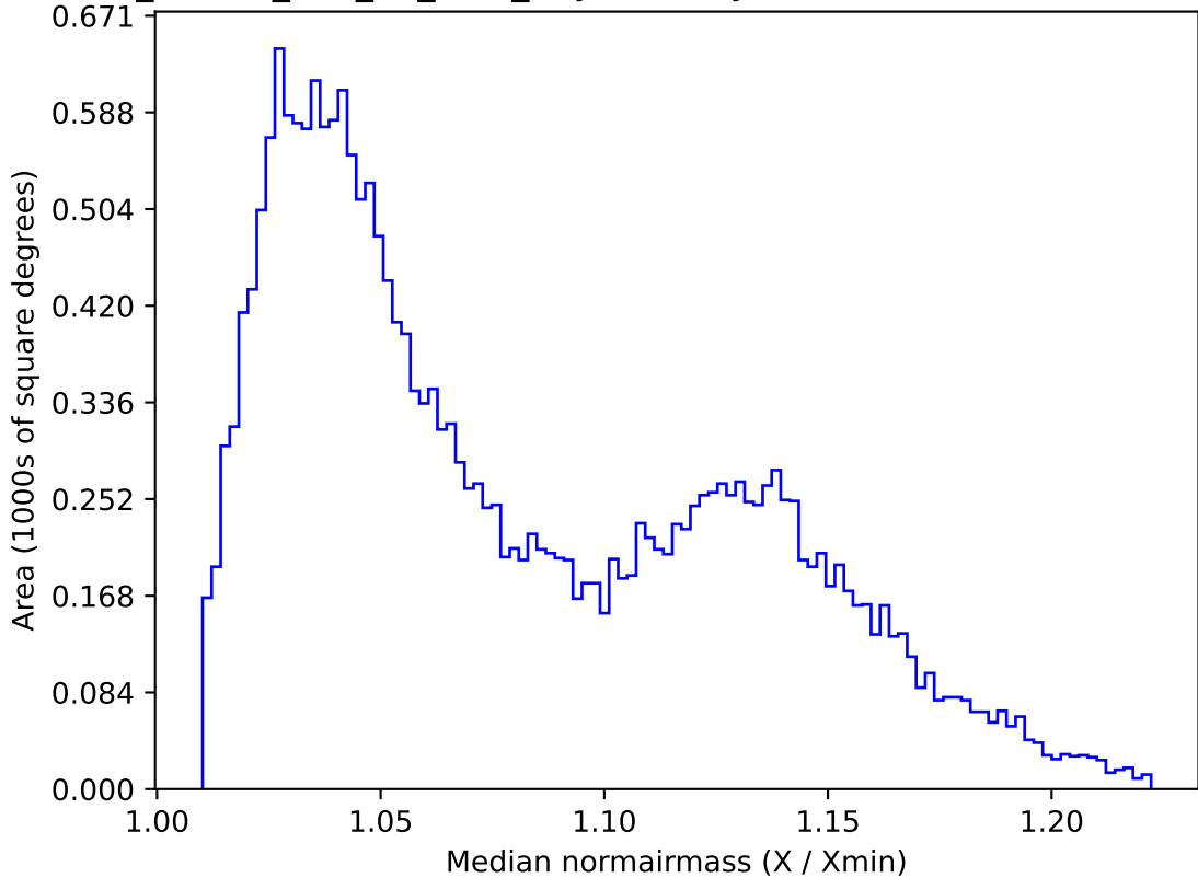
ddf_loaded_half_fl2_v3.4_10yrs All sky u band: Median normairmass
