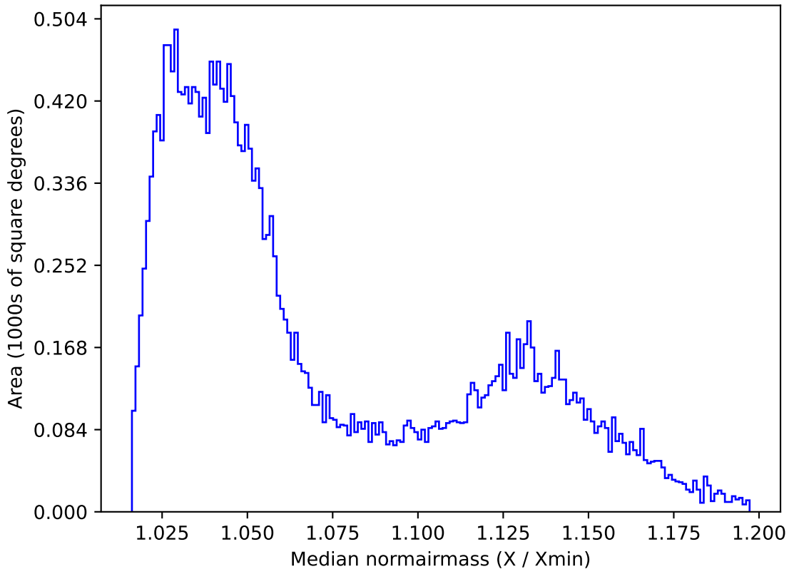
ddf_loaded_half_fl2_v3.4_10yrs All sky r band: Median normairmass
