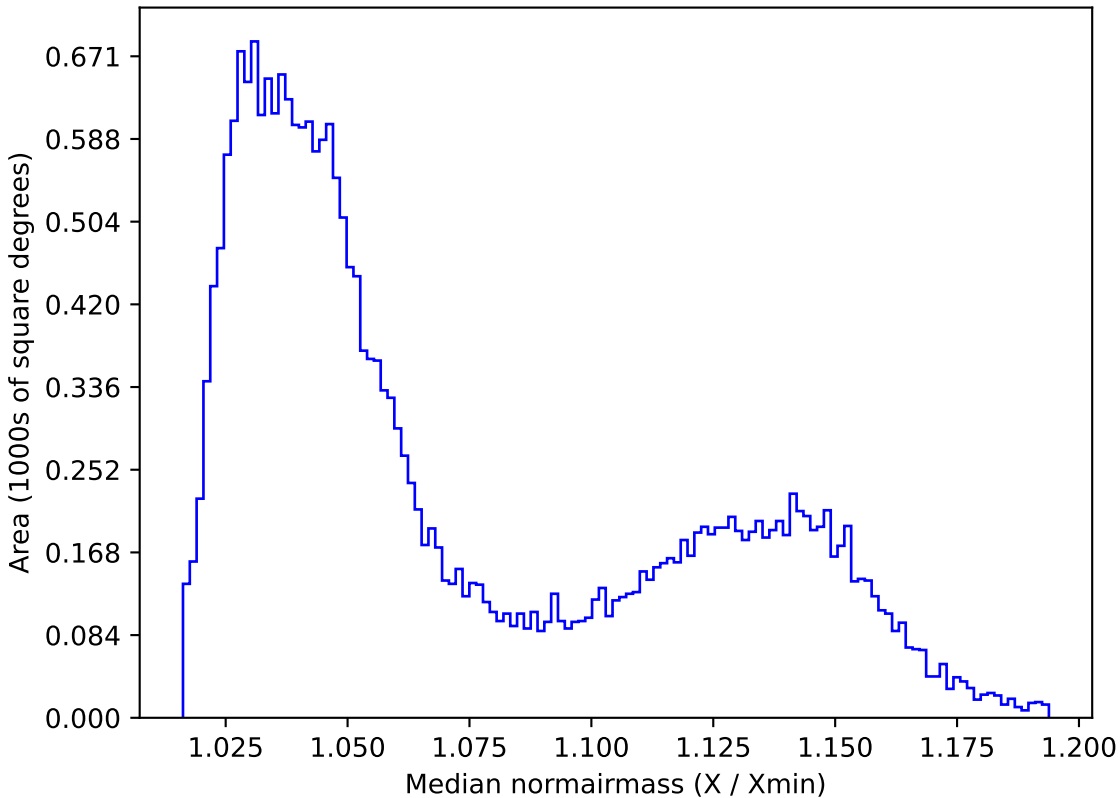
ddf_loaded_half_fl2_v3.4_10yrs All sky i band: Median normairmass
