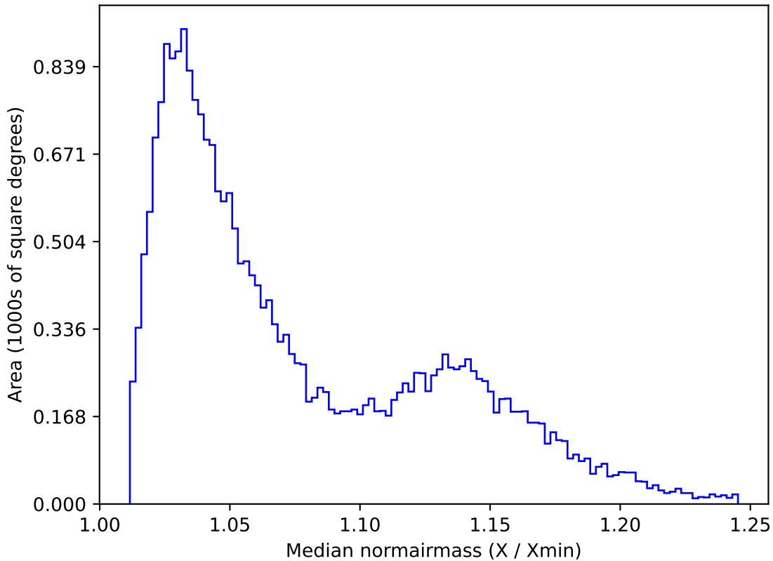
ddf_loaded_half_fl2_v3.4_10yrs All sky g band: Median normairmass
