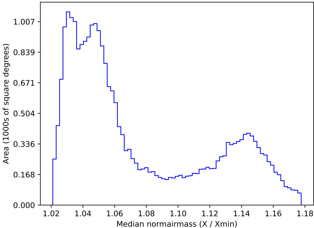
ddf_loaded_half_fl2_v3.4_10yrs All sky all bands: Median normairmass
