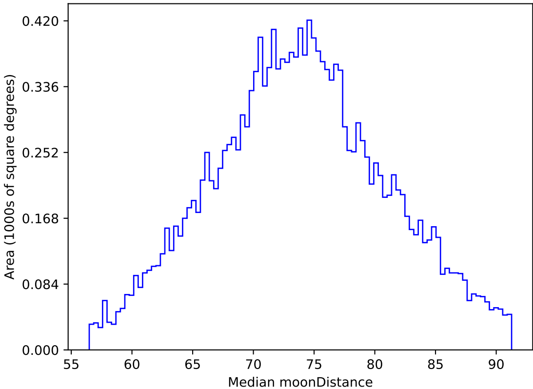
ddf_loaded_half_fl2_v3.4_10yrs WFD z band: Median moonDistance
