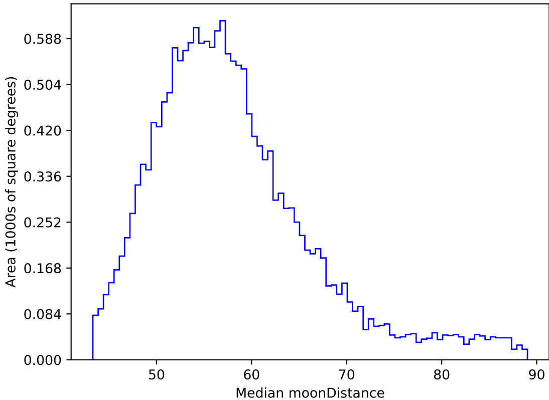
ddf_loaded_half_fl2_v3.4_10yrs WFD y band: Median moonDistance
