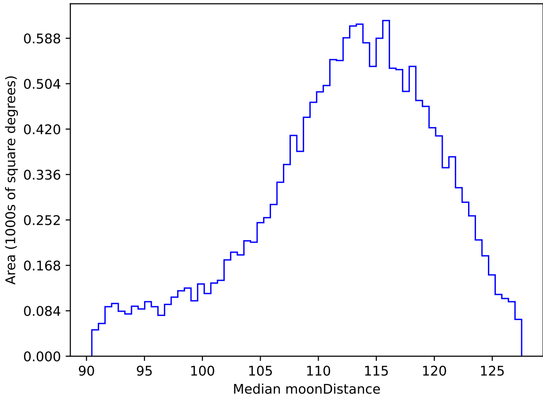
ddf_loaded_half_fl2_v3.4_10yrs WFD r band: Median moonDistance
