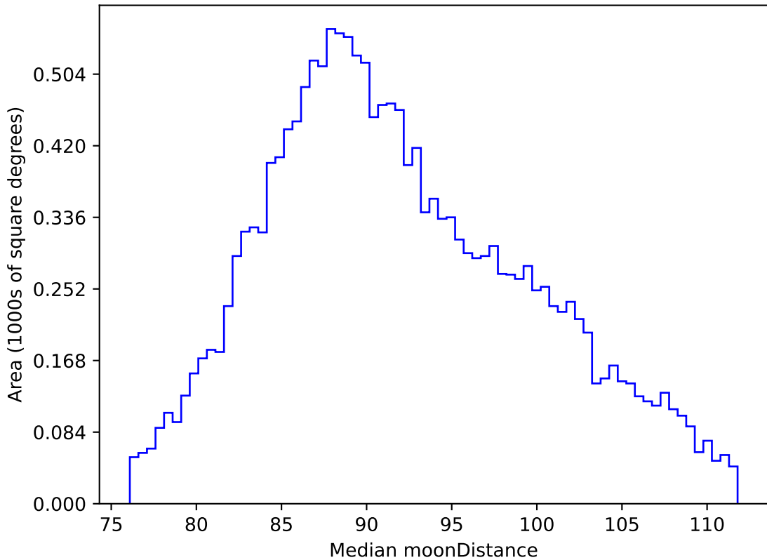
ddf_loaded_half_fl2_v3.4_10yrs WFD i band: Median moonDistance
