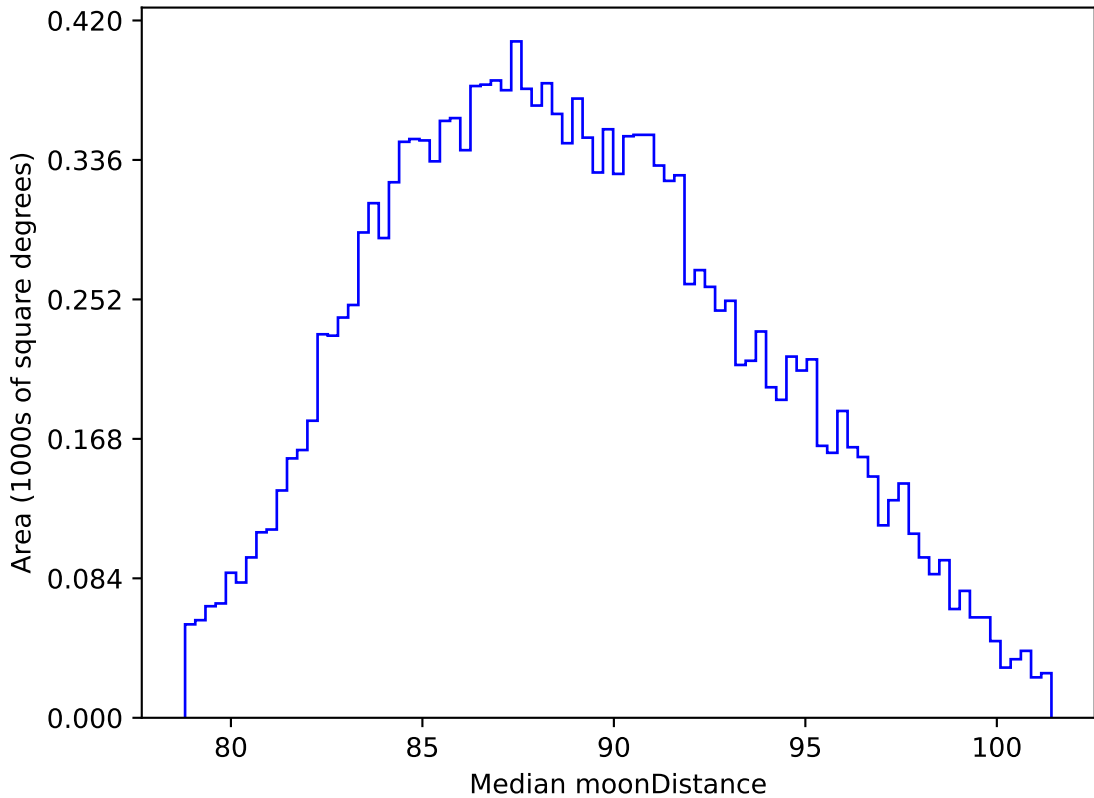
ddf_loaded_half_fl2_v3.4_10yrs WFD all bands: Median moonDistance
