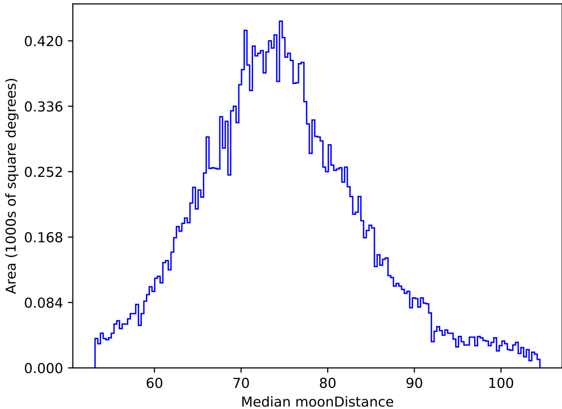
ddf_loaded_half_fl2_v3.4_10yrs All sky z band: Median moonDistance
