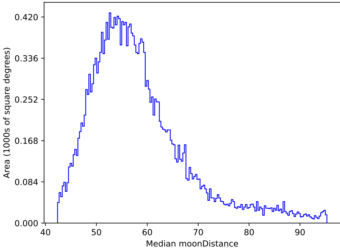
ddf_loaded_half_fl2_v3.4_10yrs All sky y band: Median moonDistance
