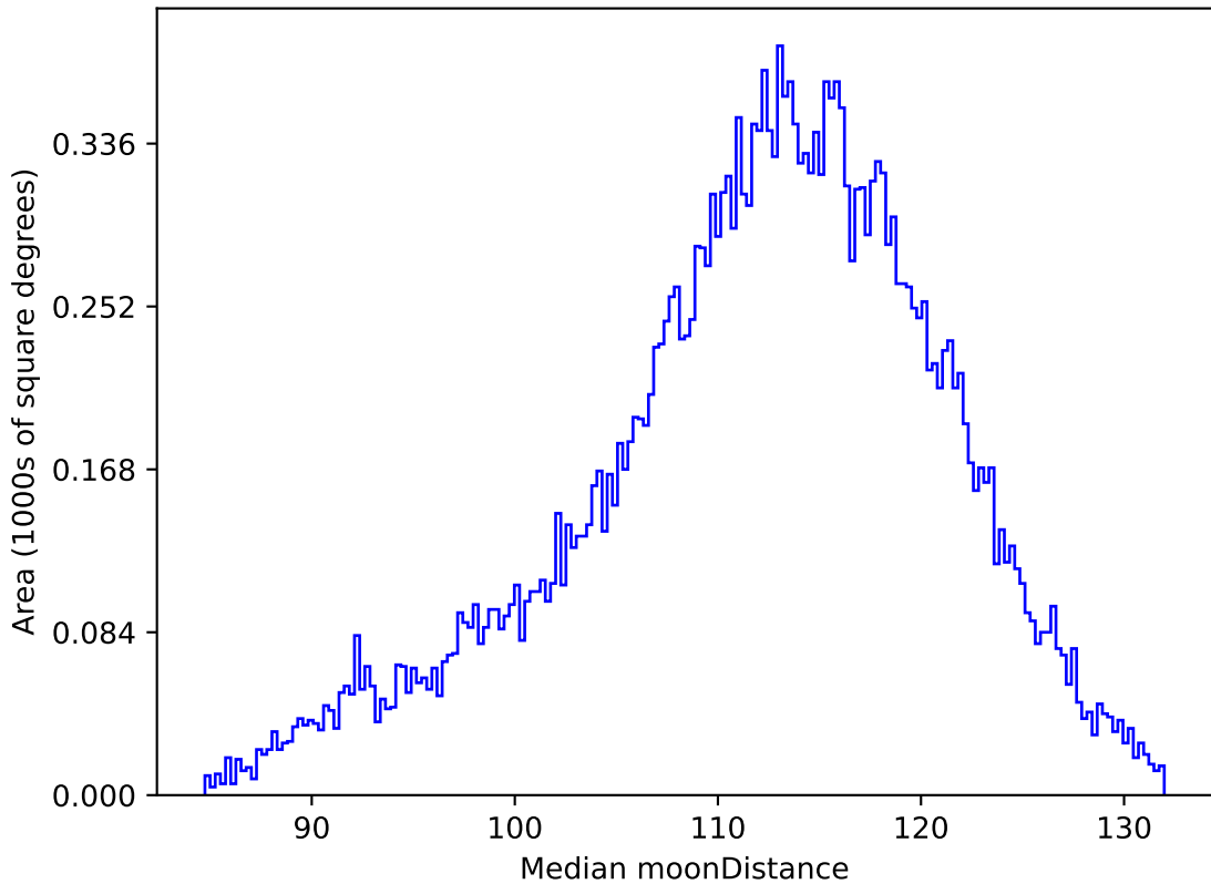
ddf_loaded_half_fl2_v3.4_10yrs All sky r band: Median moonDistance
