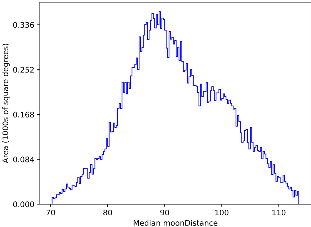
ddf_loaded_half_fl2_v3.4_10yrs All sky i band: Median moonDistance
