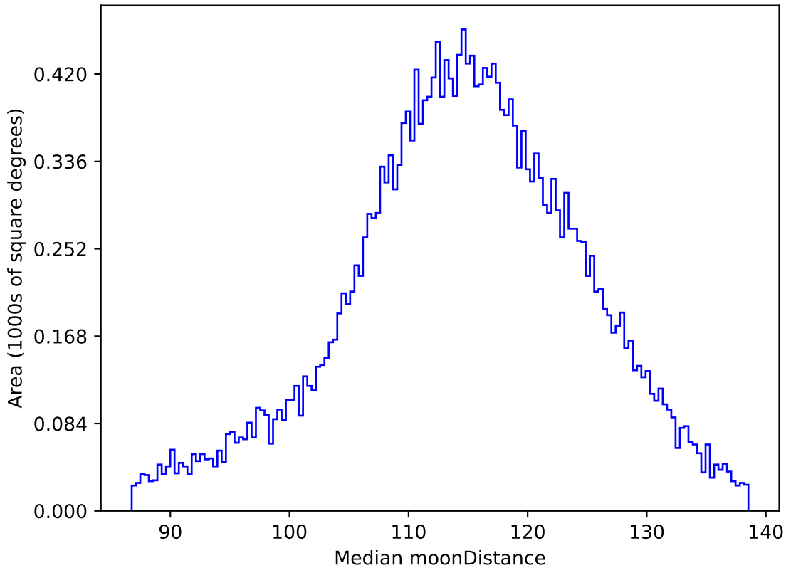
ddf_loaded_half_fl2_v3.4_10yrs All sky g band: Median moonDistance
