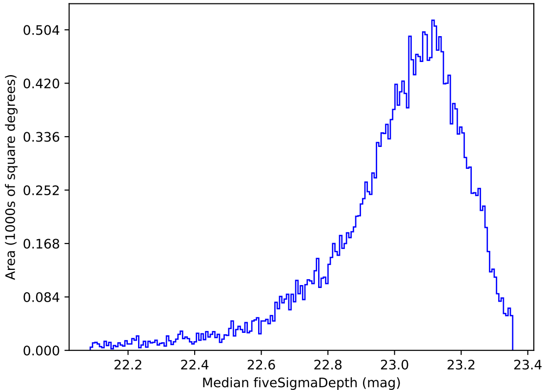
ddf_loaded_half_fl2_v3.4_10yrs Yr 1 z band: Median fiveSigmaDepth
