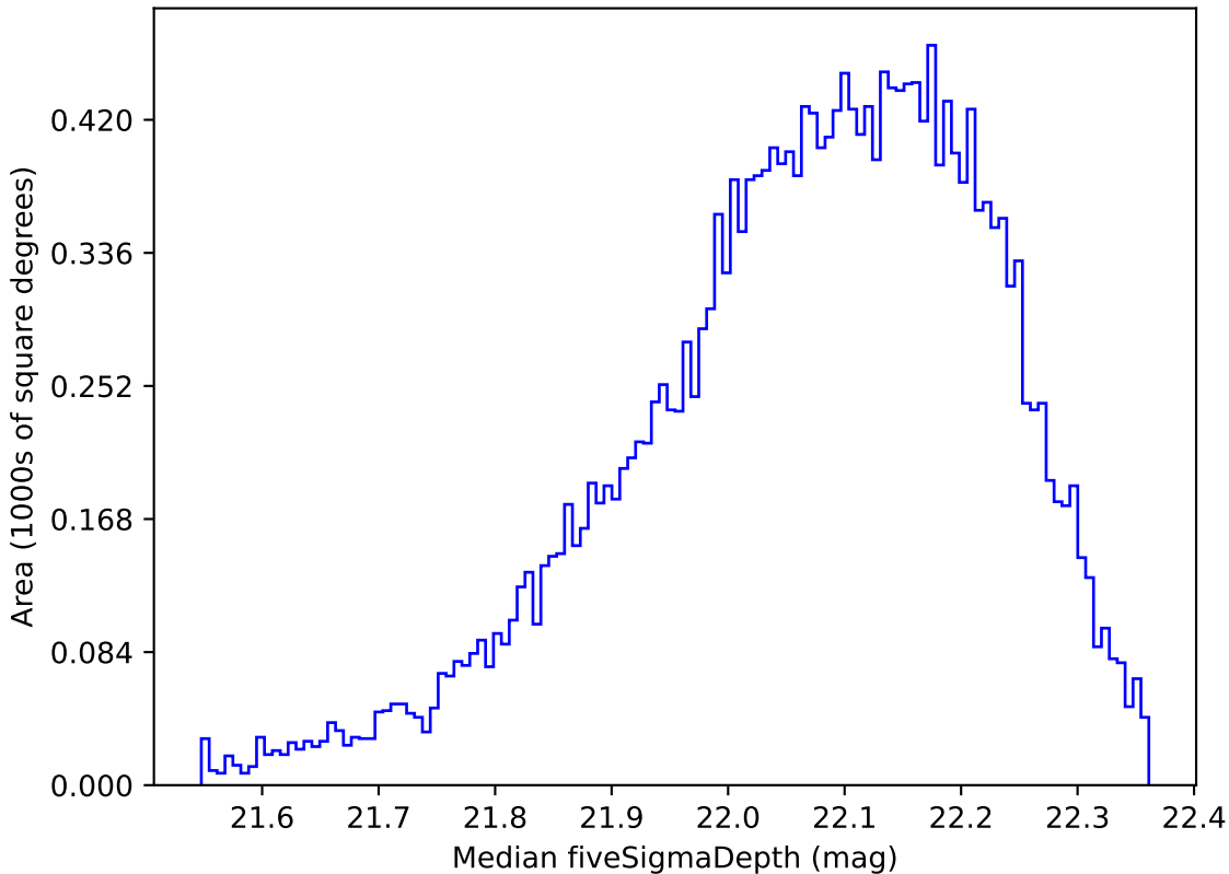
ddf_loaded_half_fl2_v3.4_10yrs Yr 1 y band: Median fiveSigmaDepth
