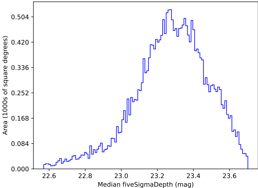
ddf_loaded_half_fl2_v3.4_10yrs Yr 1 u band: Median fiveSigmaDepth
