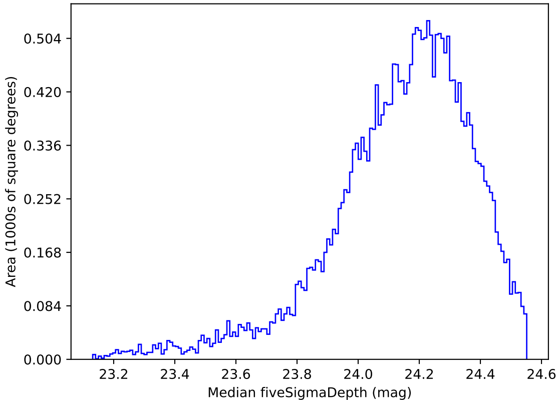
ddf_loaded_half_fl2_v3.4_10yrs Yr 1 r band: Median fiveSigmaDepth
