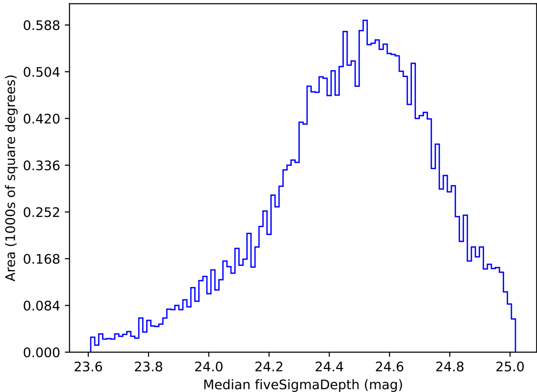
ddf_loaded_half_fl2_v3.4_10yrs Yr 1 g band: Median fiveSigmaDepth
