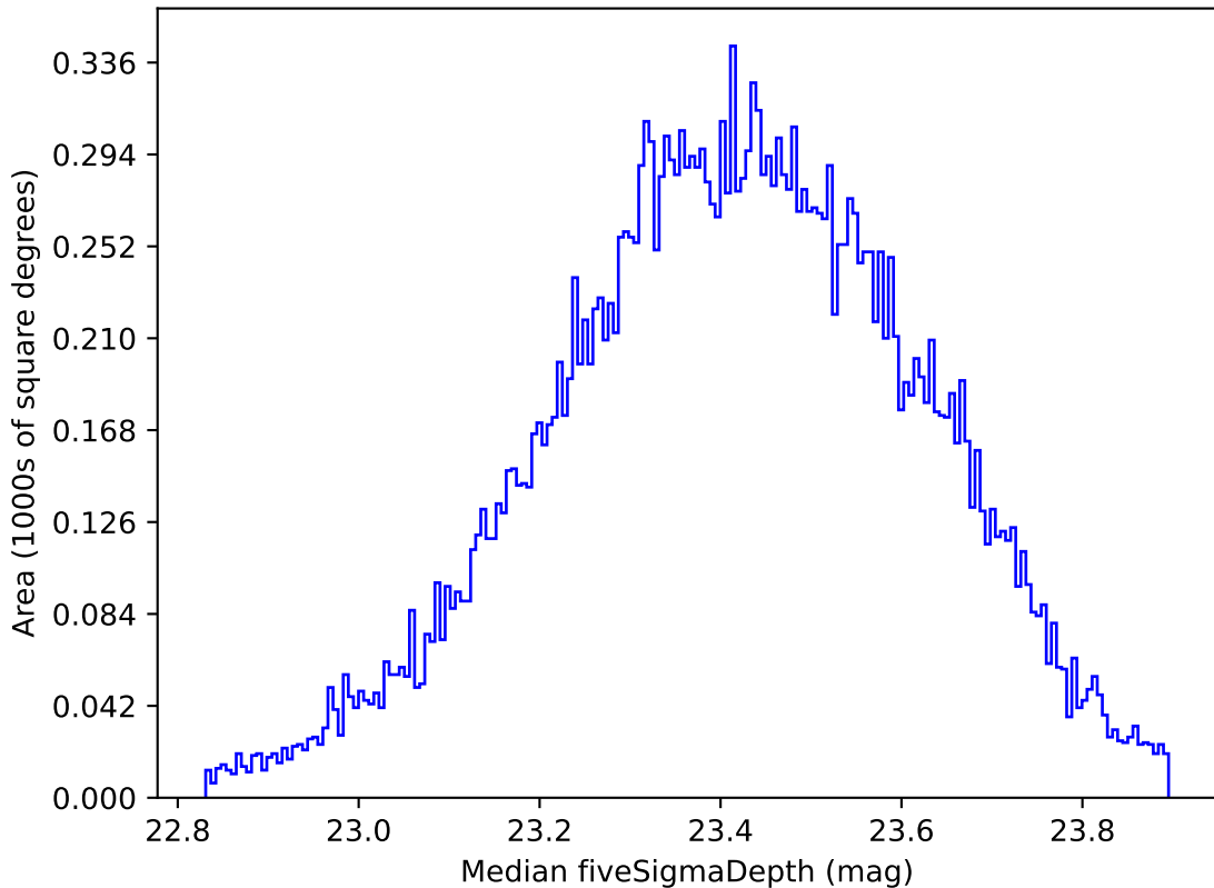
ddf_loaded_half_fl2_v3.4_10yrs Yr 1 all bands: Median fiveSigmaDepth
