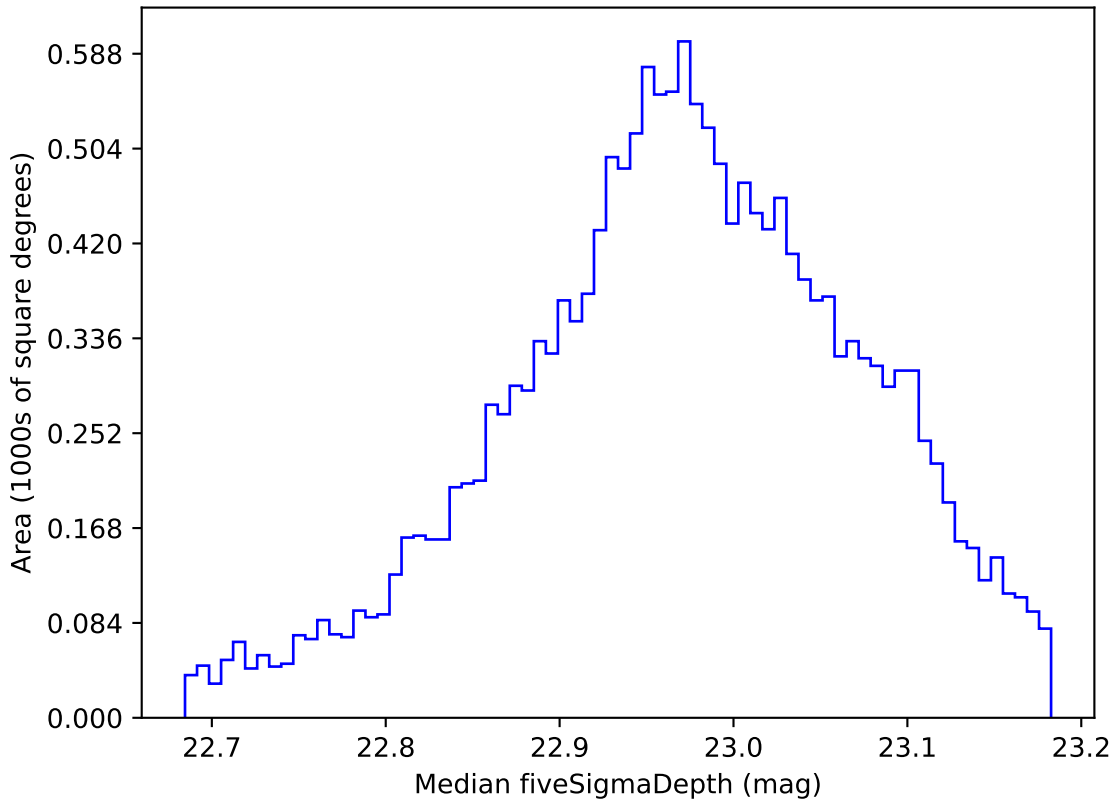
ddf_loaded_half_fl2_v3.4_10yrs WFD z band: Median fiveSigmaDepth
