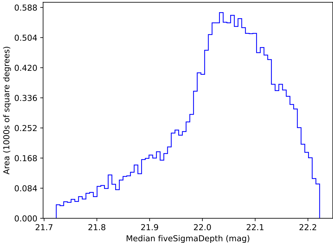
ddf_loaded_half_fl2_v3.4_10yrs WFD y band: Median fiveSigmaDepth
