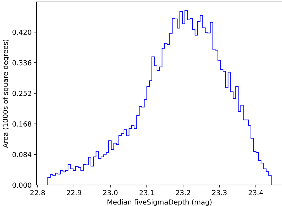
ddf_loaded_half_fl2_v3.4_10yrs WFD u band: Median fiveSigmaDepth
