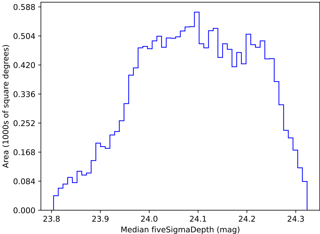
ddf_loaded_half_fl2_v3.4_10yrs WFD r band: Median fiveSigmaDepth
