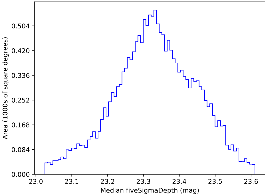
ddf_loaded_half_fl2_v3.4_10yrs WFD all bands: Median fiveSigmaDepth
