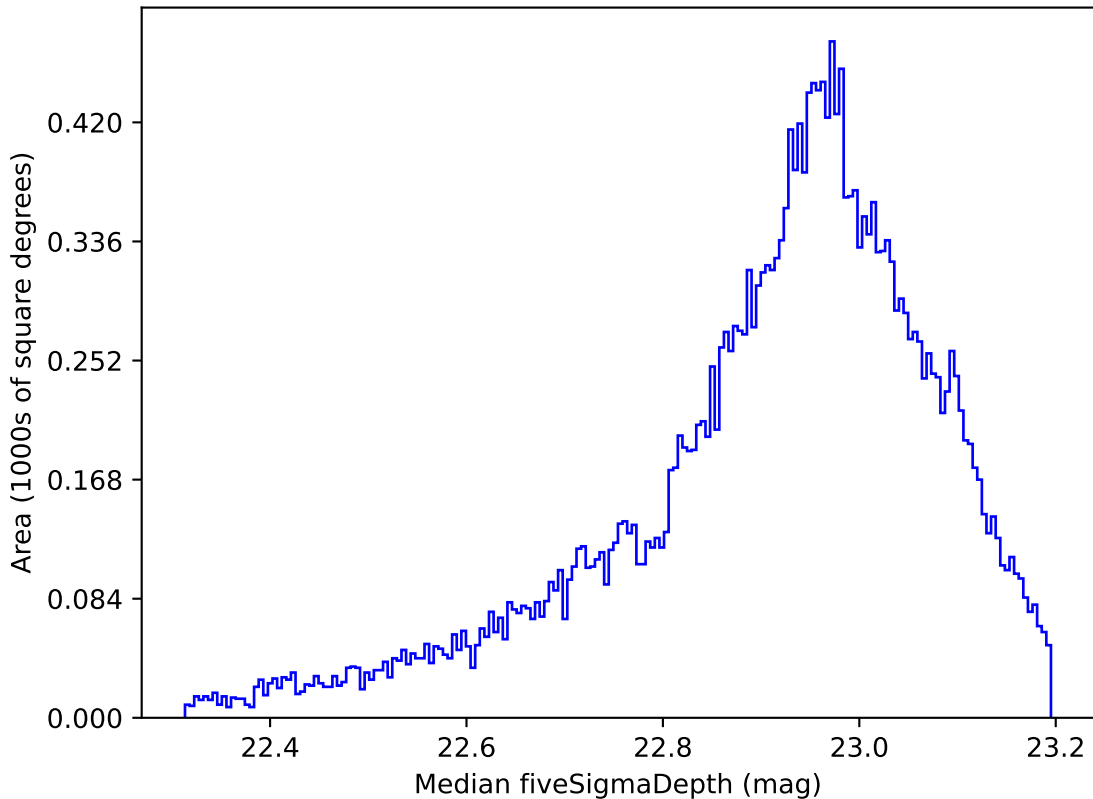
ddf_loaded_half_fl2_v3.4_10yrs All sky z band: Median fiveSigmaDepth
