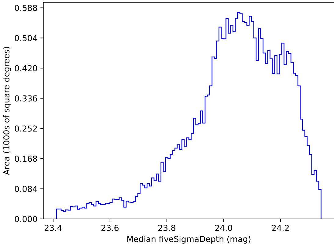
ddf_loaded_half_fl2_v3.4_10yrs All sky r band: Median fiveSigmaDepth
