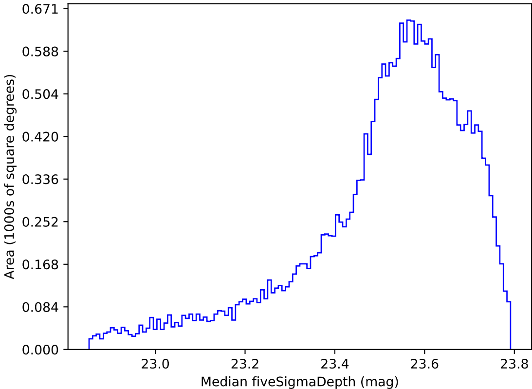
ddf_loaded_half_fl2_v3.4_10yrs All sky i band: Median fiveSigmaDepth
