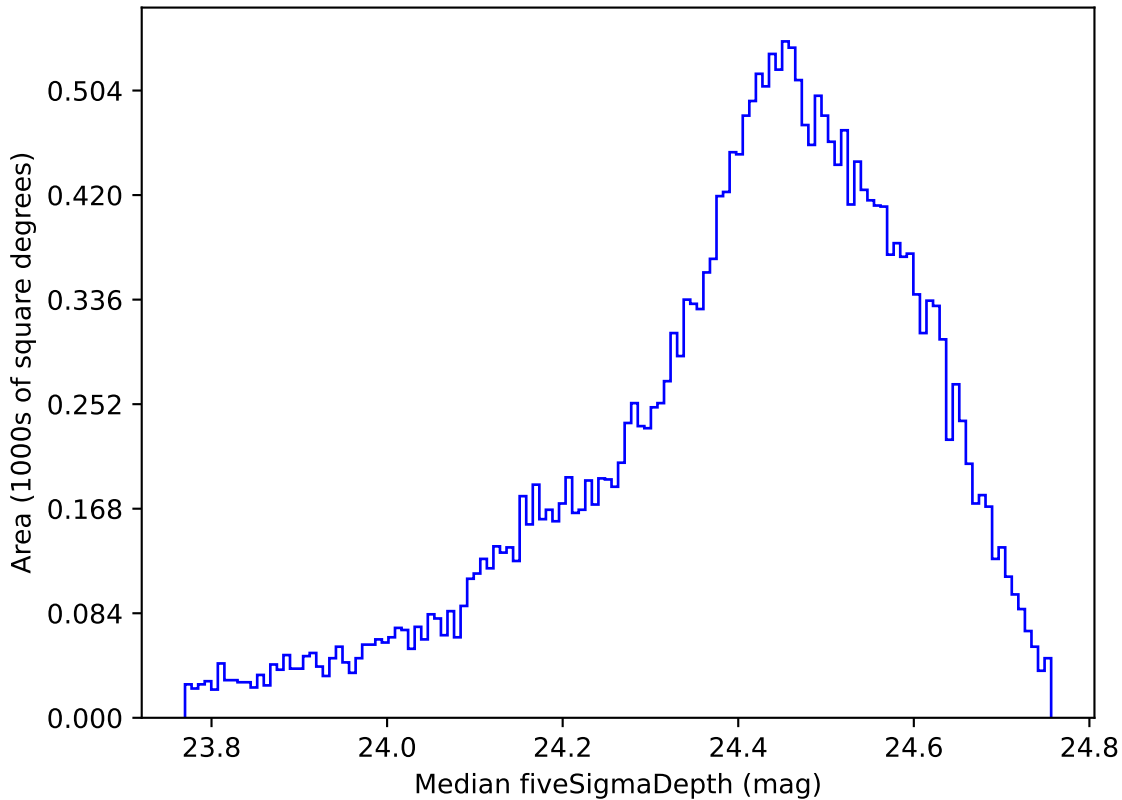
ddf_loaded_half_fl2_v3.4_10yrs All sky g band: Median fiveSigmaDepth
