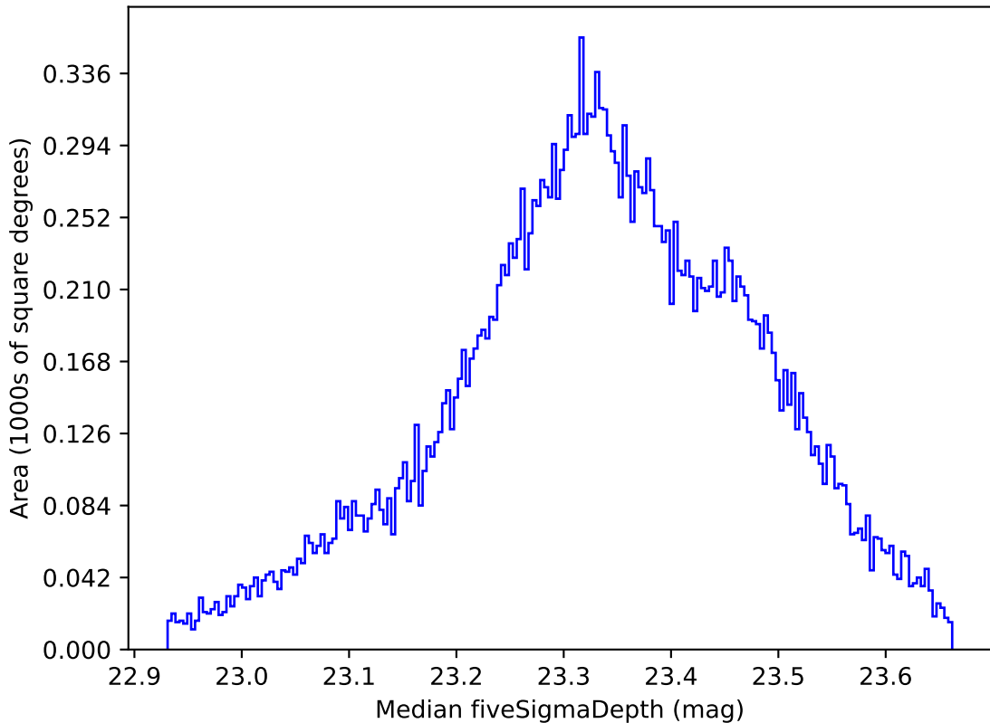
ddf_loaded_half_fl2_v3.4_10yrs All sky all bands: Median fiveSigmaDepth
