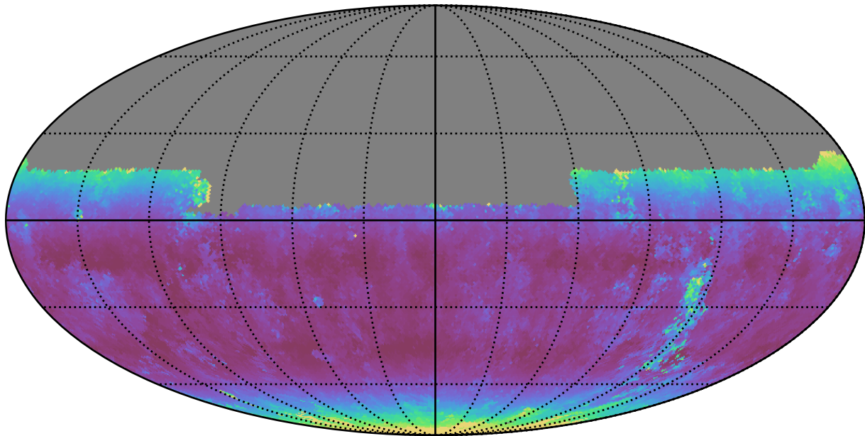
ddf_loaded_half_fl2_v3.4_10yrs Yr 1 y band: Median airmass
