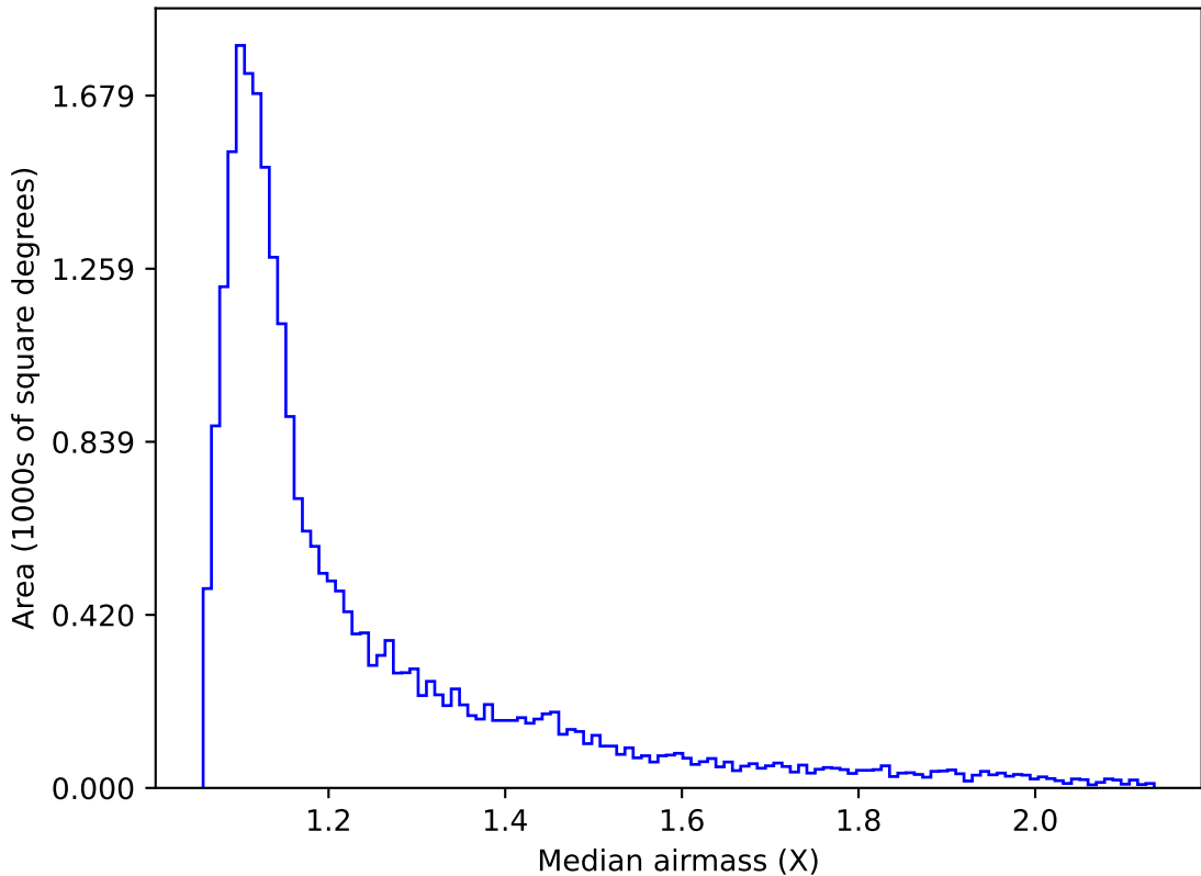
ddf_loaded_half_fl2_v3.4_10yrs Yr 1 r band: Median airmass
