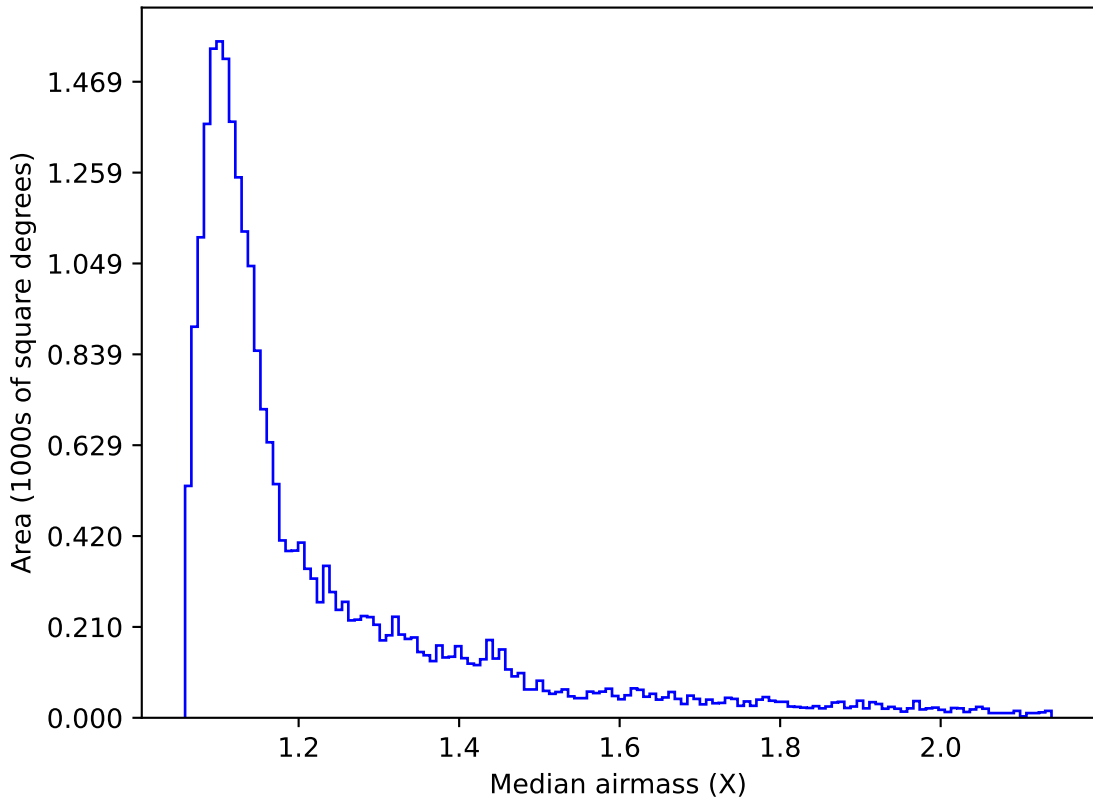
ddf_loaded_half_fl2_v3.4_10yrs Yr 1 i band: Median airmass
