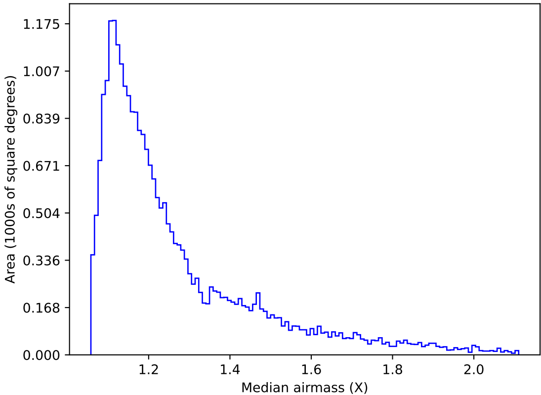
ddf_loaded_half_fl2_v3.4_10yrs Yr 1 g band: Median airmass
