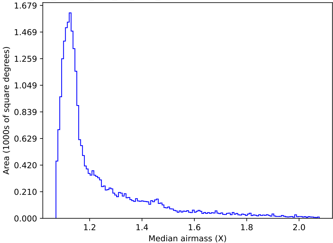
ddf_loaded_half_fl2_v3.4_10yrs Yr 1 all bands: Median airmass
