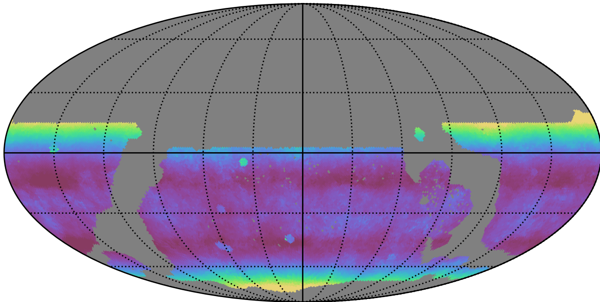
ddf_loaded_half_fl2_v3.4_10yrs WFD z band: Median airmass
