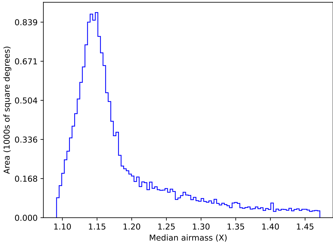
ddf_loaded_half_f12_v3.4_10yrs WFD y band: Median airmass
