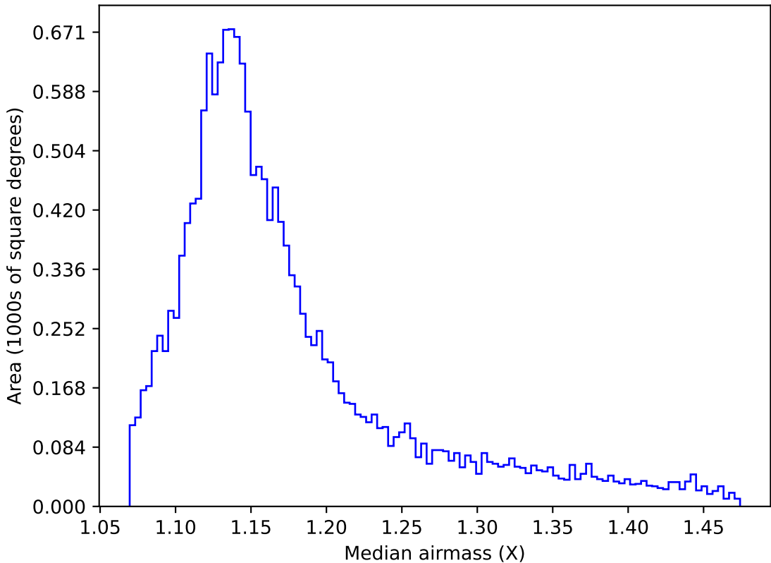
ddf_loaded_half_fi2_v3.4_10yrs WFD u band: Median airmass
